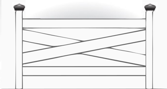
CROSSBUCK 10-1/2 spacing Post spacing 91" on center, fence height 60"
